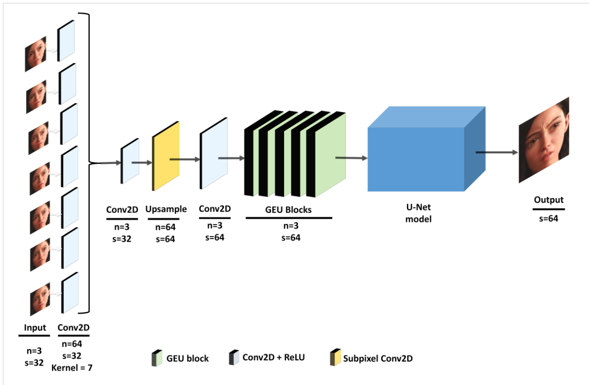
Fig. 1: Unet+GEU2 method
