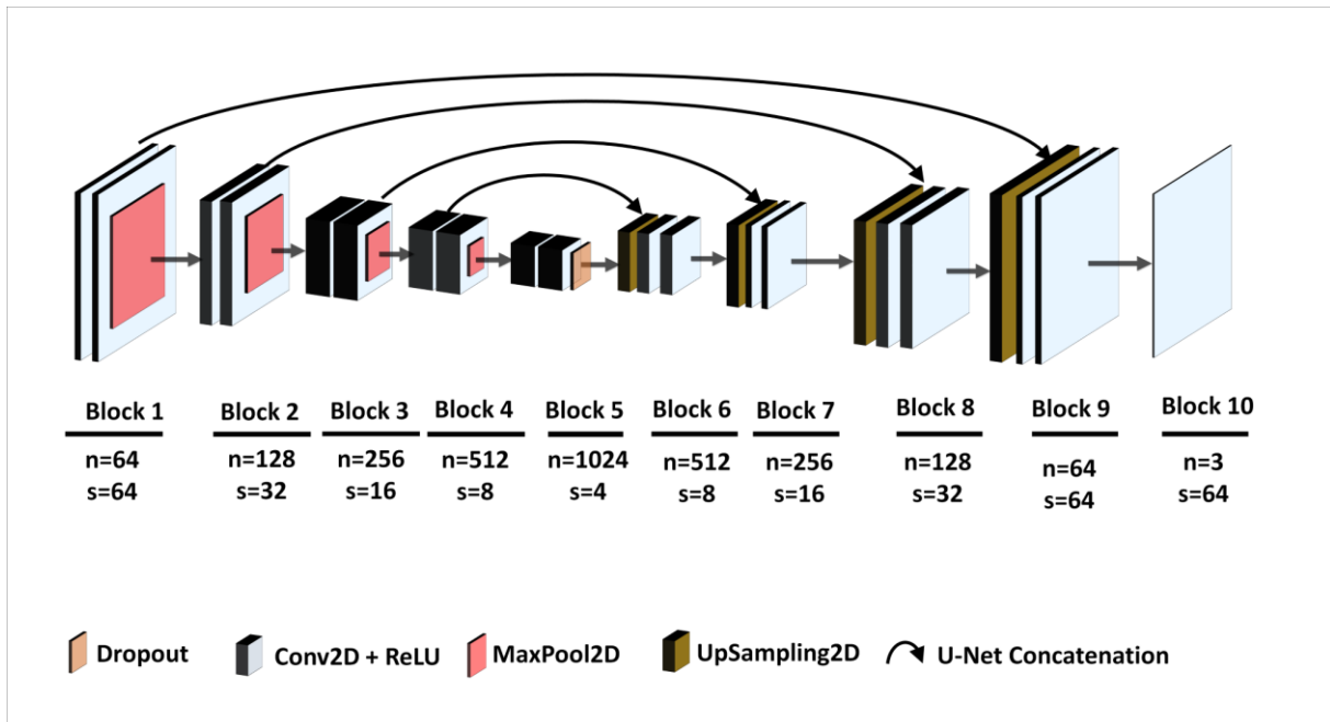
Fig. 2: U-net model
